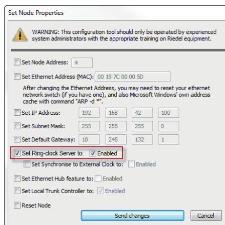
図 30 : Director - Online View - Ring Clock Server を稼働
