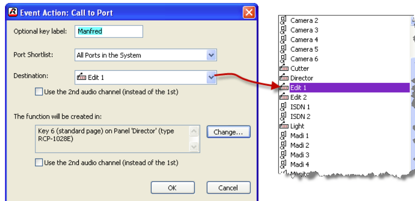
図 814 : Events – Event Action : Call to Port
