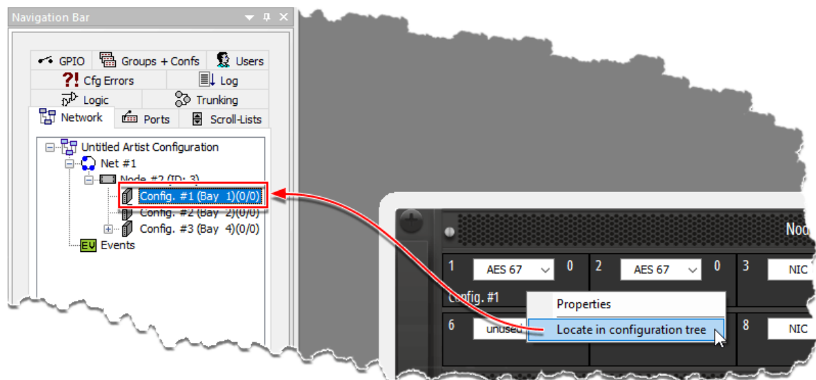
図 45：Locate in configuration tree
