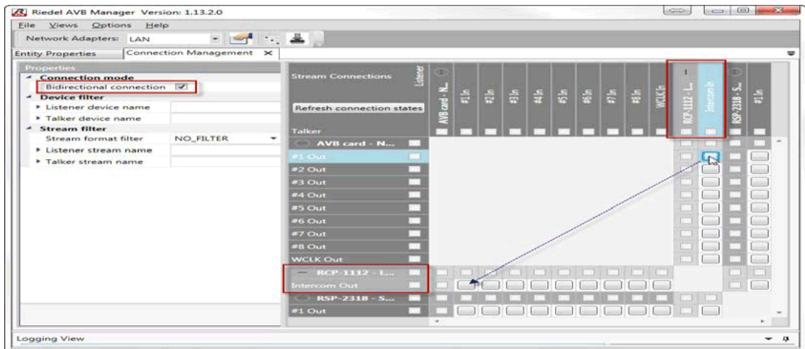
図 523 : AVB-Manager – Connection Management
