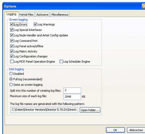
図 251 : Logging – Settings / Options / Logging
