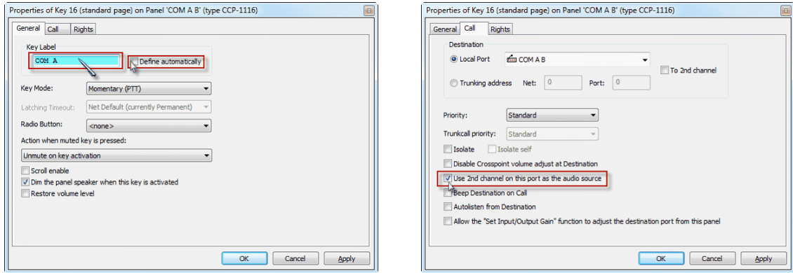
図 659 : CCP 1116 – Setup Commentator B → A
